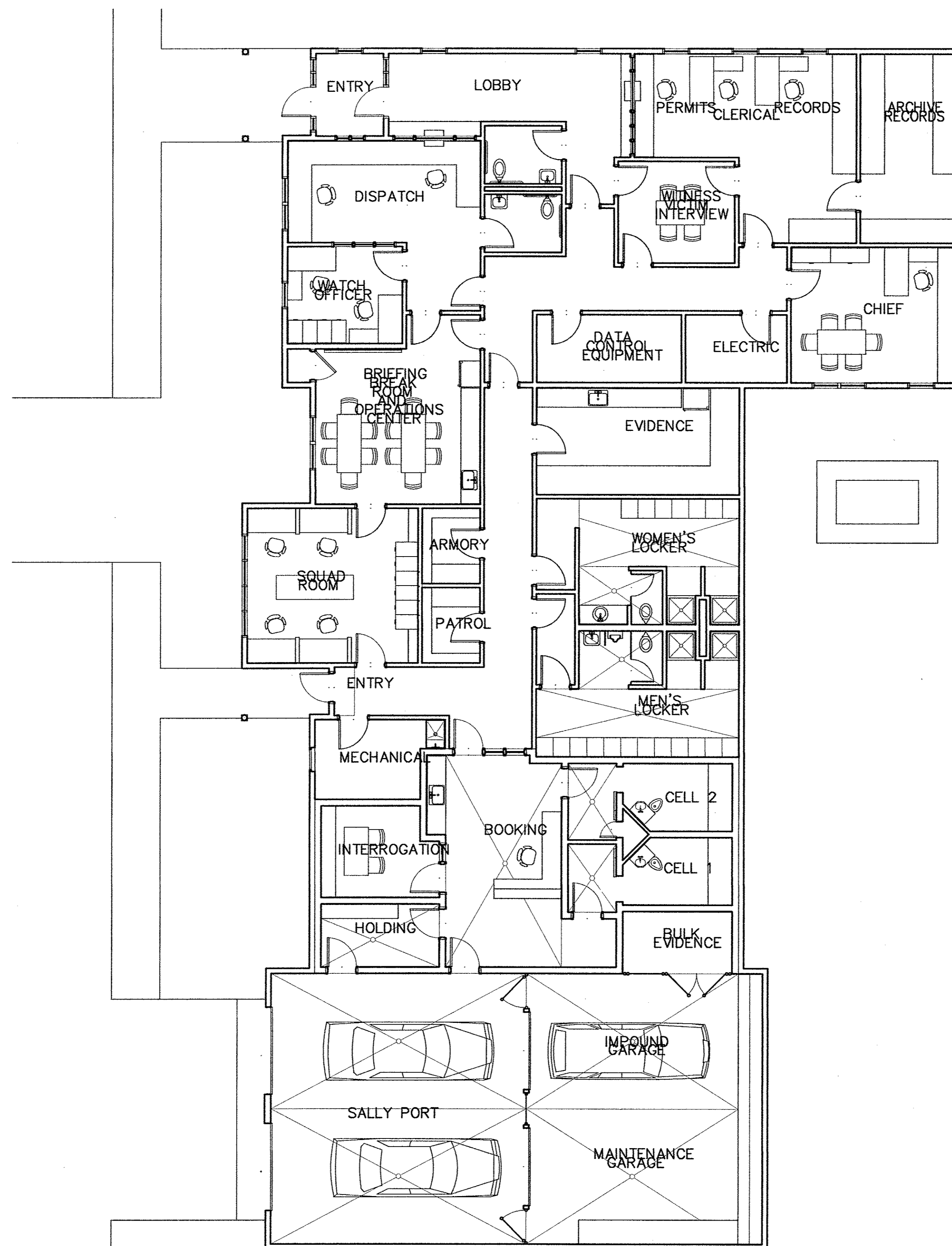
FLOOR PLAN 0 2 4 8 12
